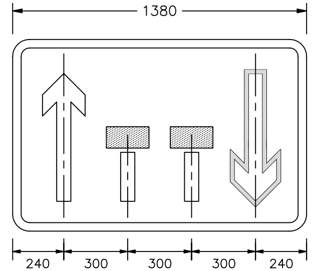
Four lane carriageway
