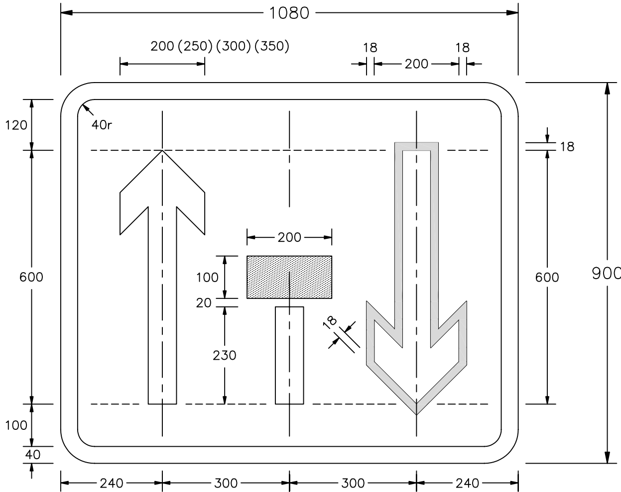
Three lane carriageway
