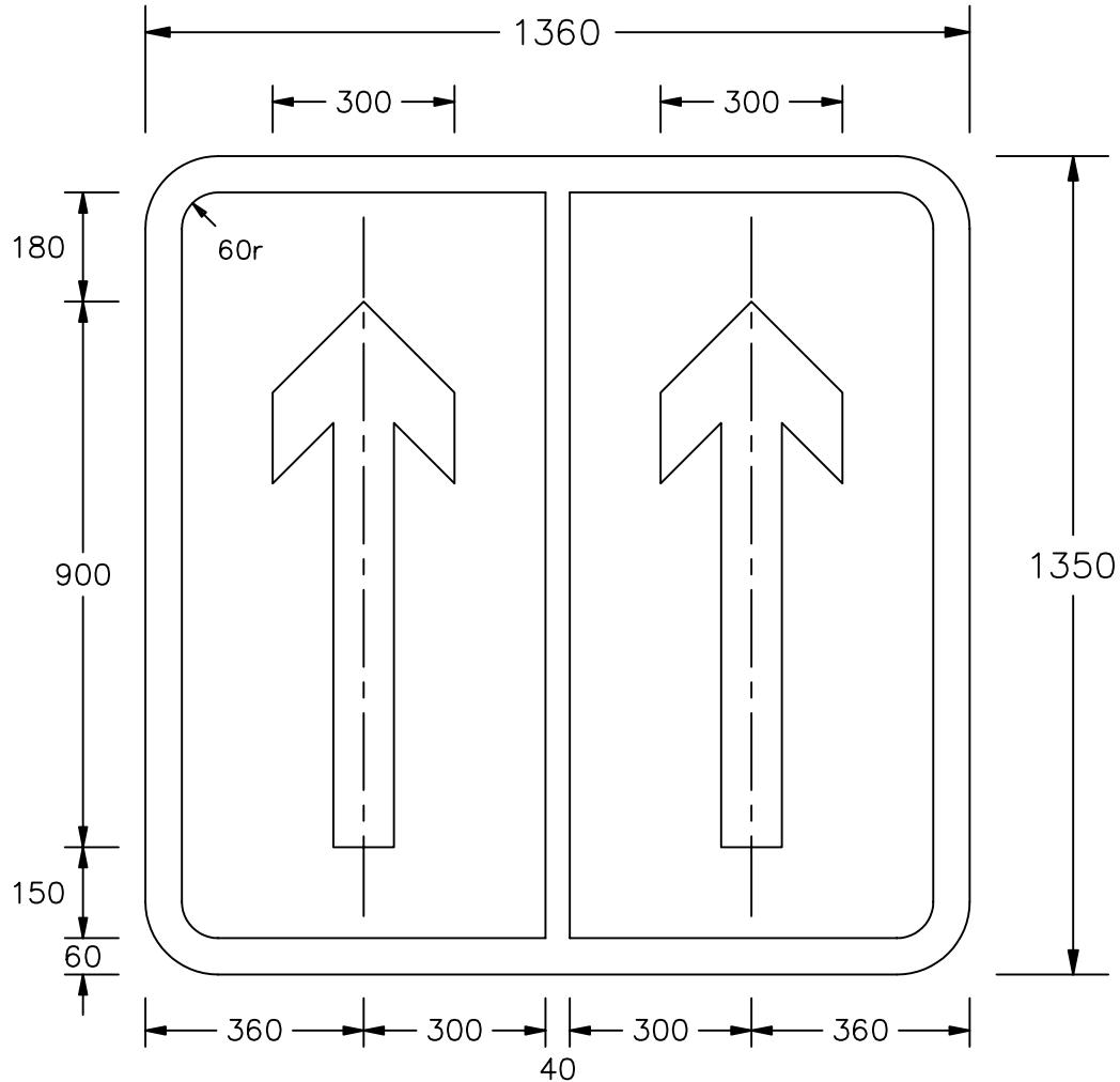
Single lane carriageway plus hard shoulder
