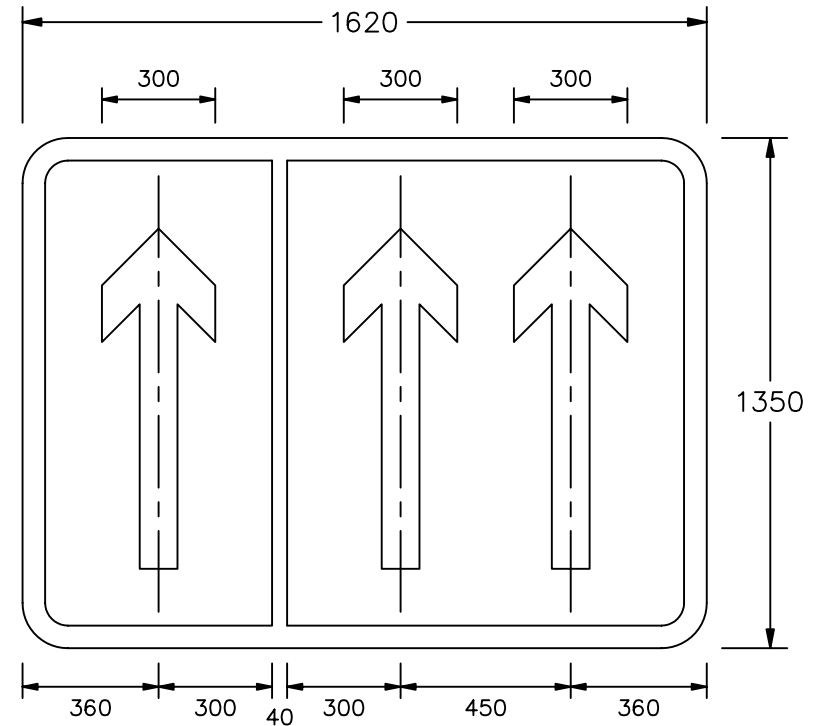
Two lane carriageway plus hard shoulder
