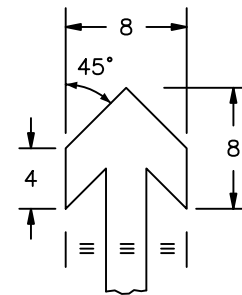
ARROW DETAILS
