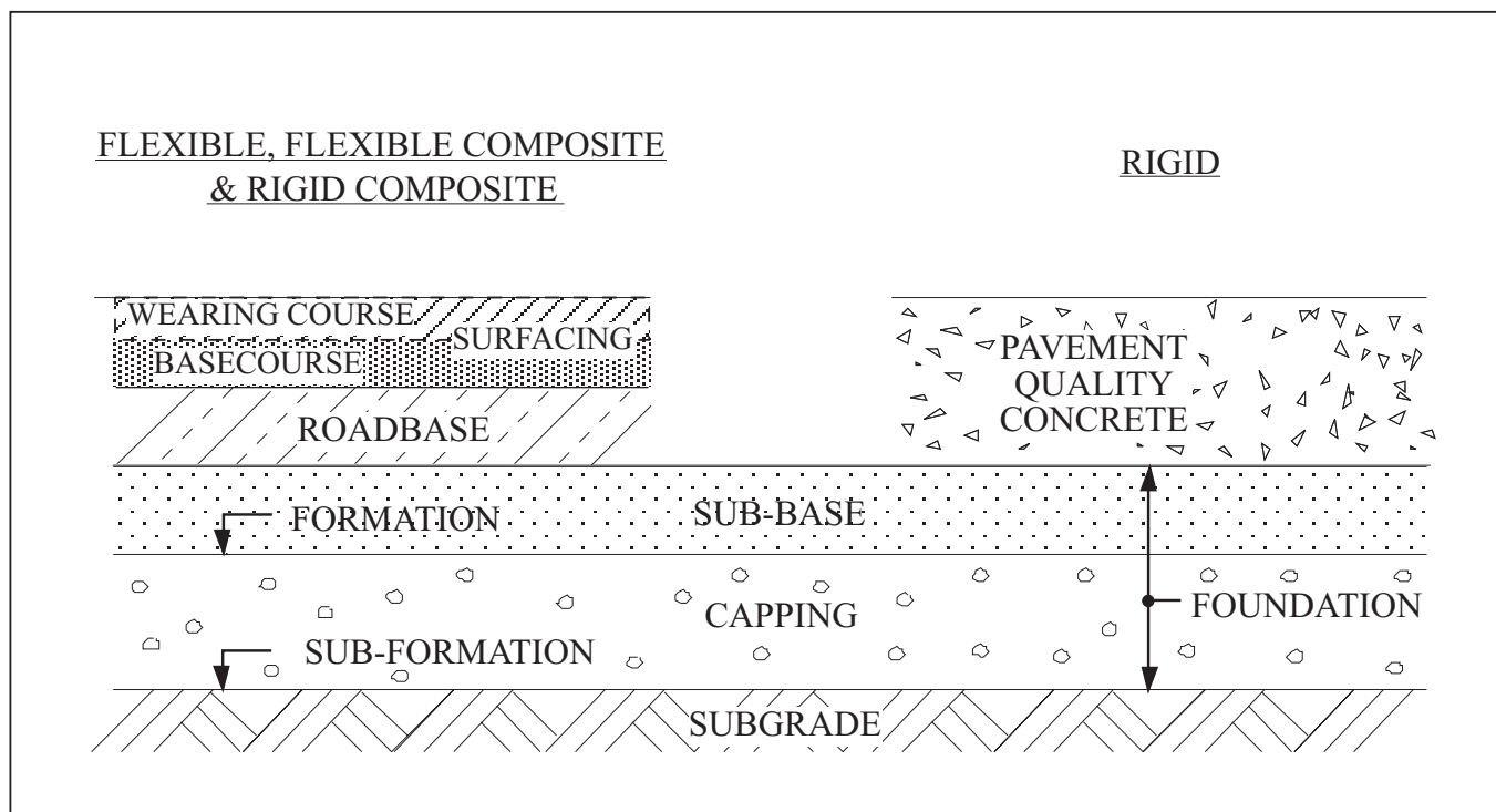
Figure 2.1 Typical Pavement
